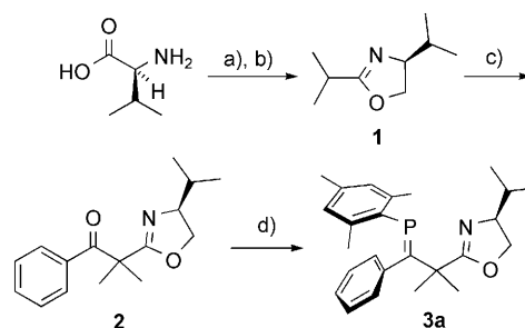
Scheme 2. Synthesis of phosphaalkene ligand. a) \text{NaBH}_4 , \text{I}_2 , THF, 60^\circ\text{C} , 18 h (92%); b) isobutyric acid, xylenes, 130^\circ\text{C} (58%); c) 1. s BuLi, TMEDA, THF, -78^\circ\text{C} ; 2. ethyl benzoate, THF, -78^\circ\text{C} to 25^\circ\text{C} (49%); d) 1. \text{MesP}(\text{SiMe}_3)_2\text{Li} , THF, -78^\circ\text{C} to 25^\circ\text{C} ; 2. \text{Me}_3\text{SiCl} quench (52%). THF = tetrahydrofuran, Bu = butyl, TMEDA = N,N,N',N' -tetramethylethylenediamine, Mes = 2,4,6-trimethylphenyl.
